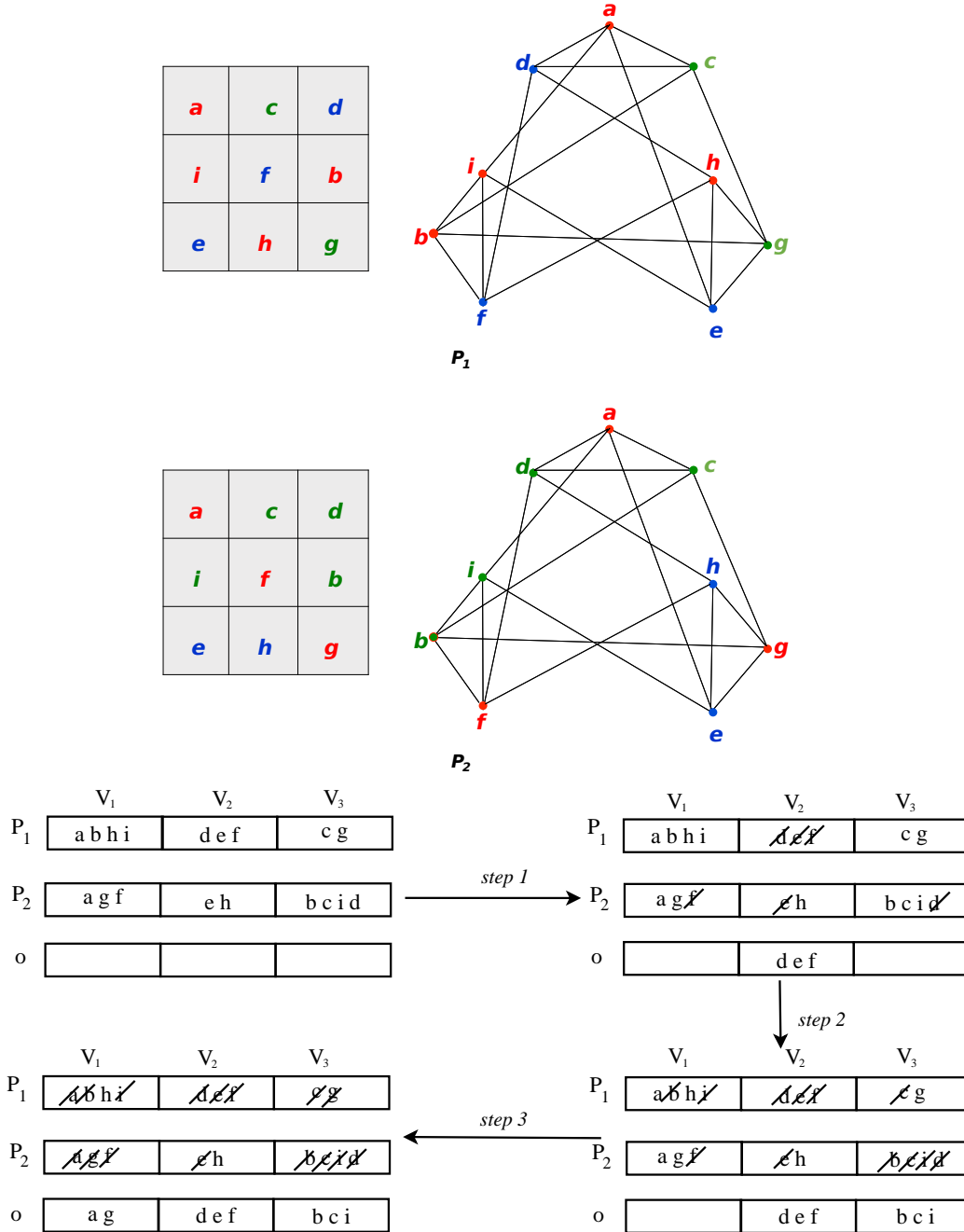
Fig. 3. Illustration of the first phase of the MAGX crossover operator (Algorithm 3 lines 2–7).
