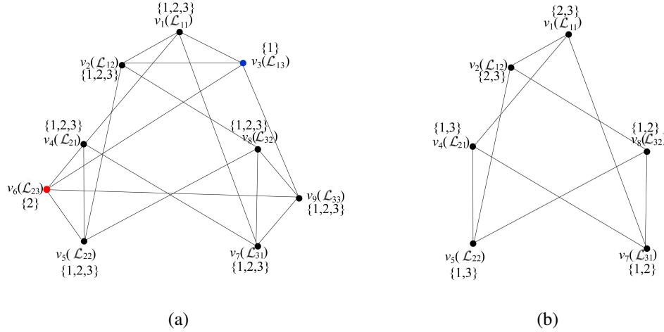
Fig. 2. The Latin square graph of Fig 1(b) and the residual Latin square graph obtained by the preprocessing procedure.
