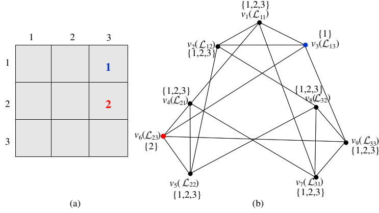
Fig. 1. An illustrative example of converting a partial Latin square (a) to a domain-constrained Latin square graph (b).
