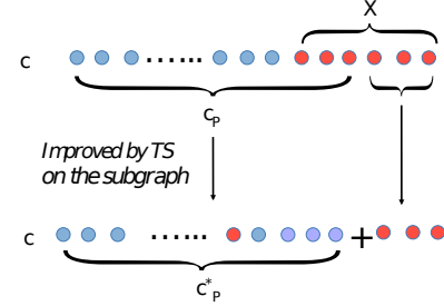
Fig. 4. The relaxation-based perturbation.
