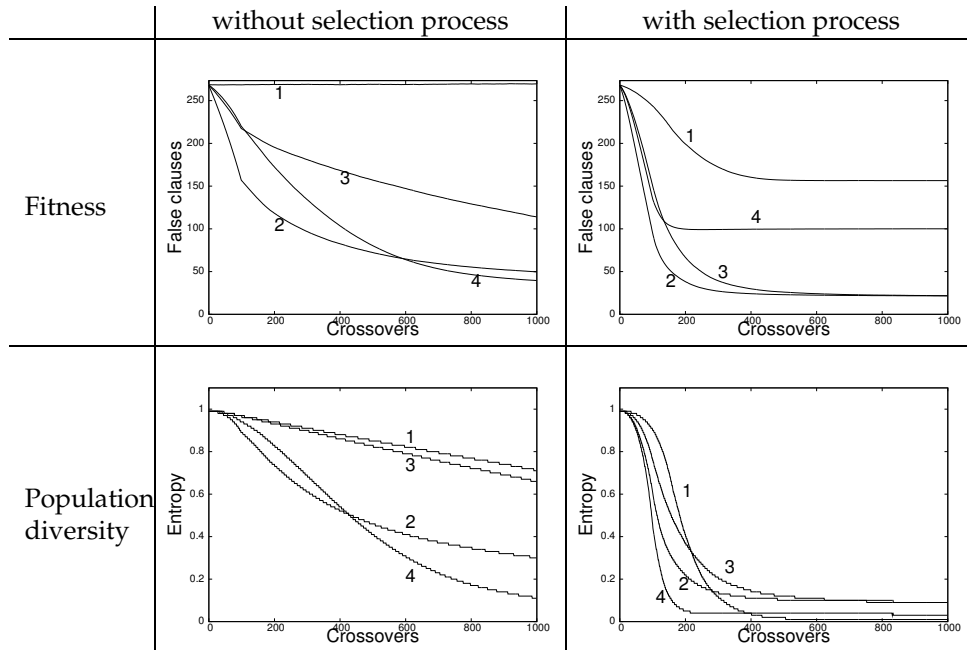
Figure 3: Evolution of the average number of false clauses and the entropy with the four crossovers (1→Uniform crossover, 2→CTM crossover, 3→CC crossover and 4→F&F crossover)
