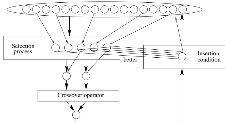
Figure 1: Selection and insertion processes. A child is obtained by a crossover between two parents randomly selected in a sub-population of the best individuals. If its fitness value is better than the value of the worst individual of the sub-population then it replaces the oldest individual of the population; otherwise the population is kept and a new selection process is executed.
