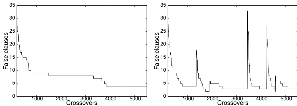
Figure 4: TS without diversity (left) and TS with diversity (right)
