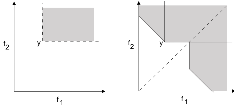
Fig. 1. P-dominated area (left). L-dominated area (right).
