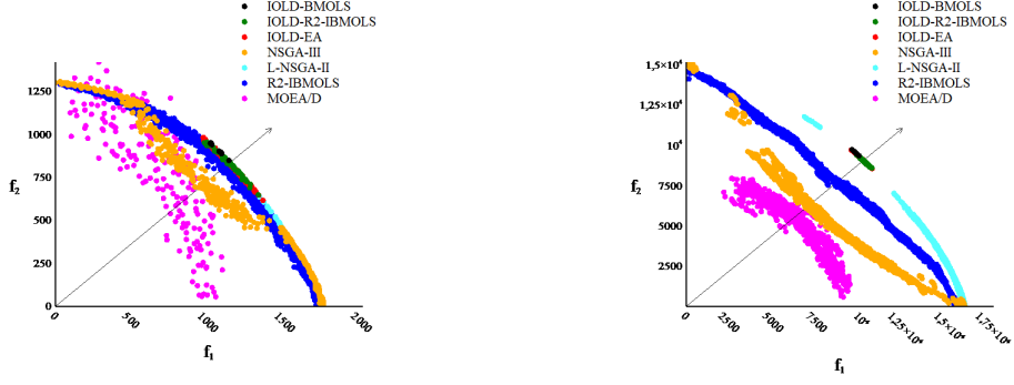
Fig. 3. Obtained solutions by the tested algorithms for the instances 2-50 (left) and 2-500 (right).
