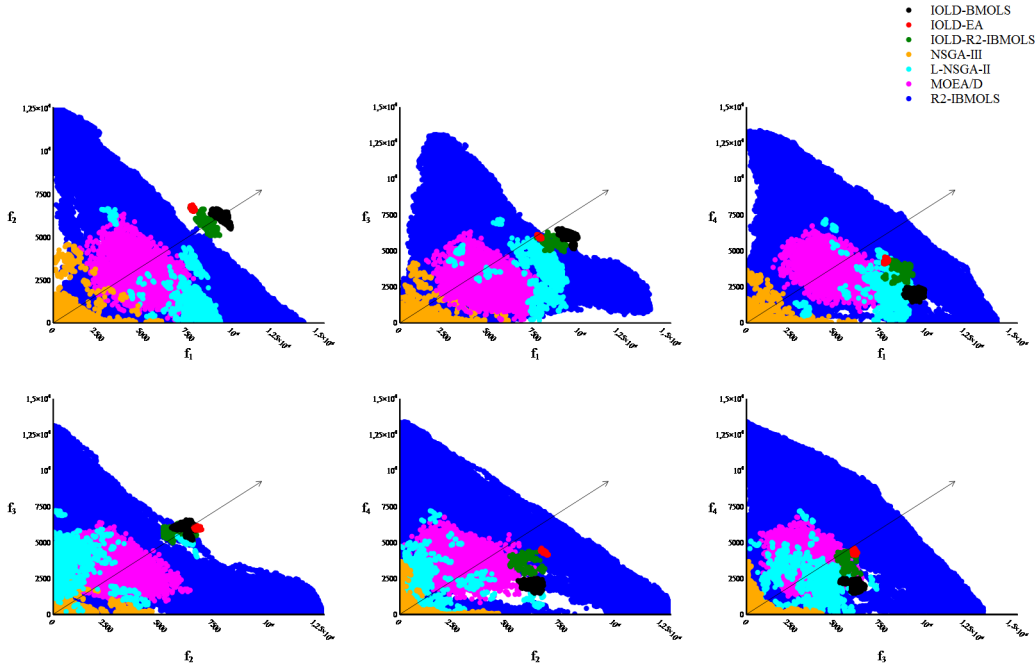
Fig. 4. Obtained solutions by the tested algorithms for the instance 4-500.
