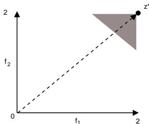
Fig. 2. Target region of the bi-objective space (gray area).
