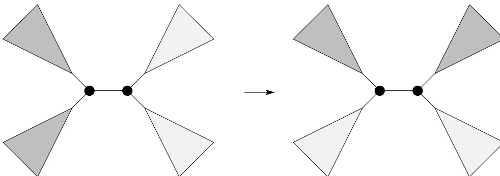
FIGURE 3.3 – Transformation NNI
